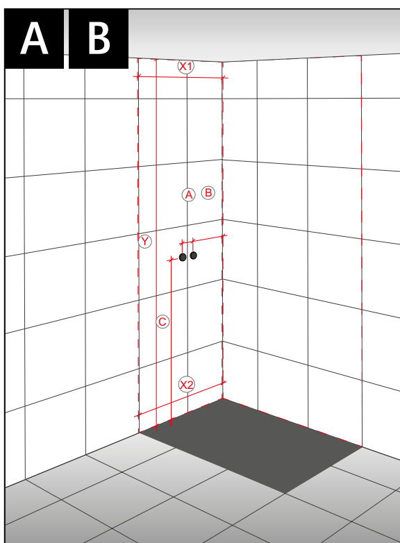
Draw the outline of the panels on the wall. Transfer the dimension onto the panel and cut the panel to size. When taking your measurements, take into account the expansion joint between the panels. Drill the holes for the connections. You can use all standard wood processing tools to work on the panels. Vacuum or sweep any shavings off the panels. Always work on the face side of the panel. Make sure that the panel is well supported. Caution - risk of breakage!
