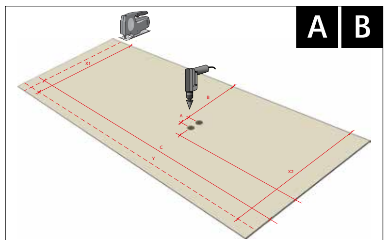
Draw the outline of the panels on the wall. Transfer the dimension onto the panel and cut the panel to size. When taking your measurements, take into account the expansion joint between the panels. Drill the holes for the connections. You can use all standard wood processing tools to work on the panels. Vacuum or sweep any shavings off the panels. Always work on the face side of the panel. Make sure that the panel is well supported. Caution - risk of breakage!
