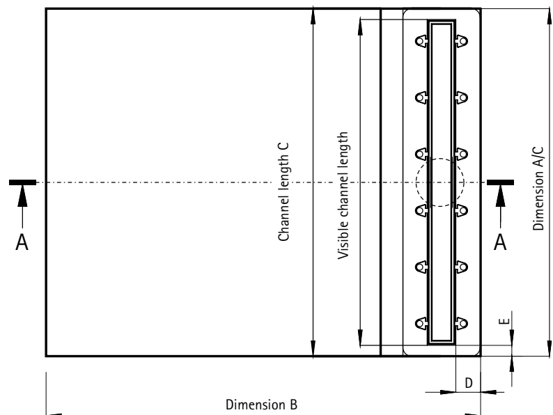
General top view LINE2K
