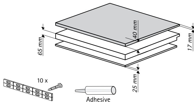
TECEdrainline Natural stone
