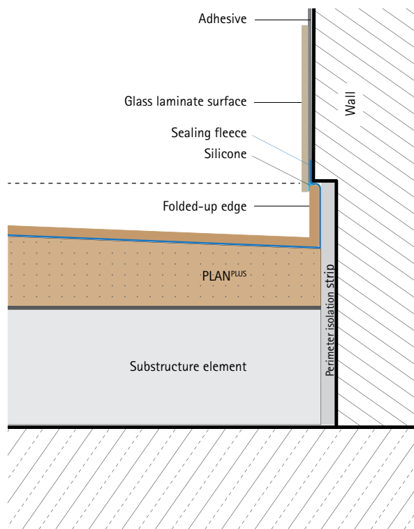
Folded-up edge with overlaid glass laminate/fleece
