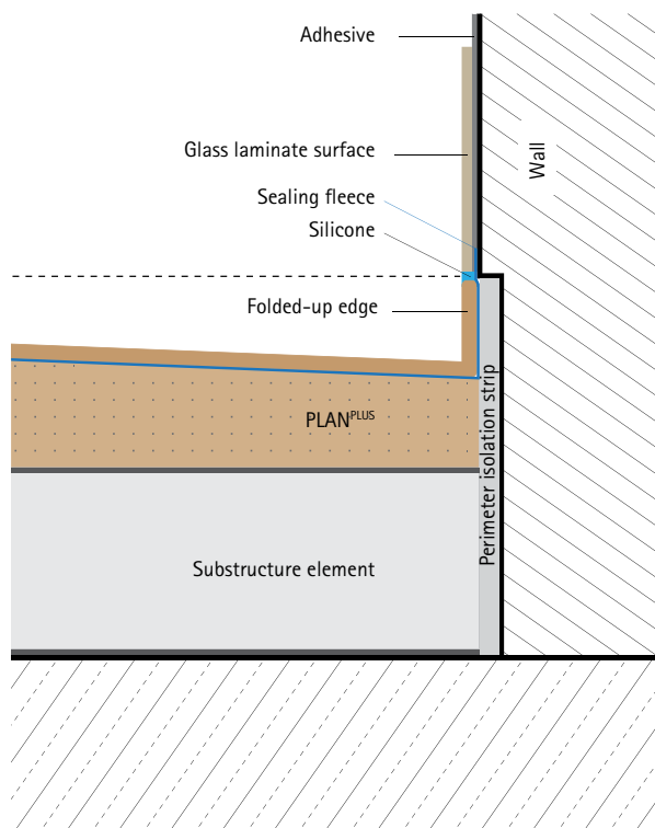
Folded-up edge with flush glass laminate/fleece
