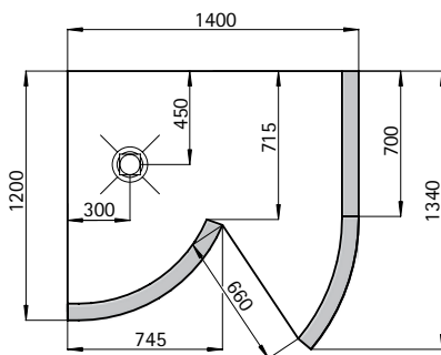
Fig. Corner 1400, entrance on right
