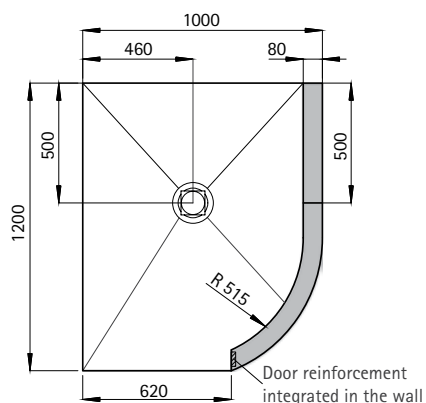
Fig. Entrance on left
