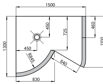
Fig. Corner 1500, entrance on right
