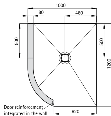
Fig. Entrance on right
