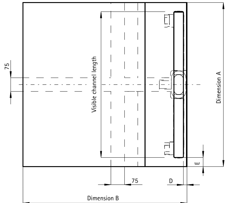
General top view LINE2DNW
