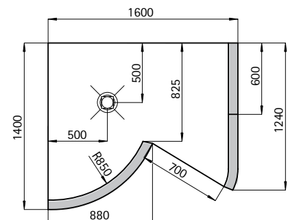
Fig. Corner 1600, entrance on right
