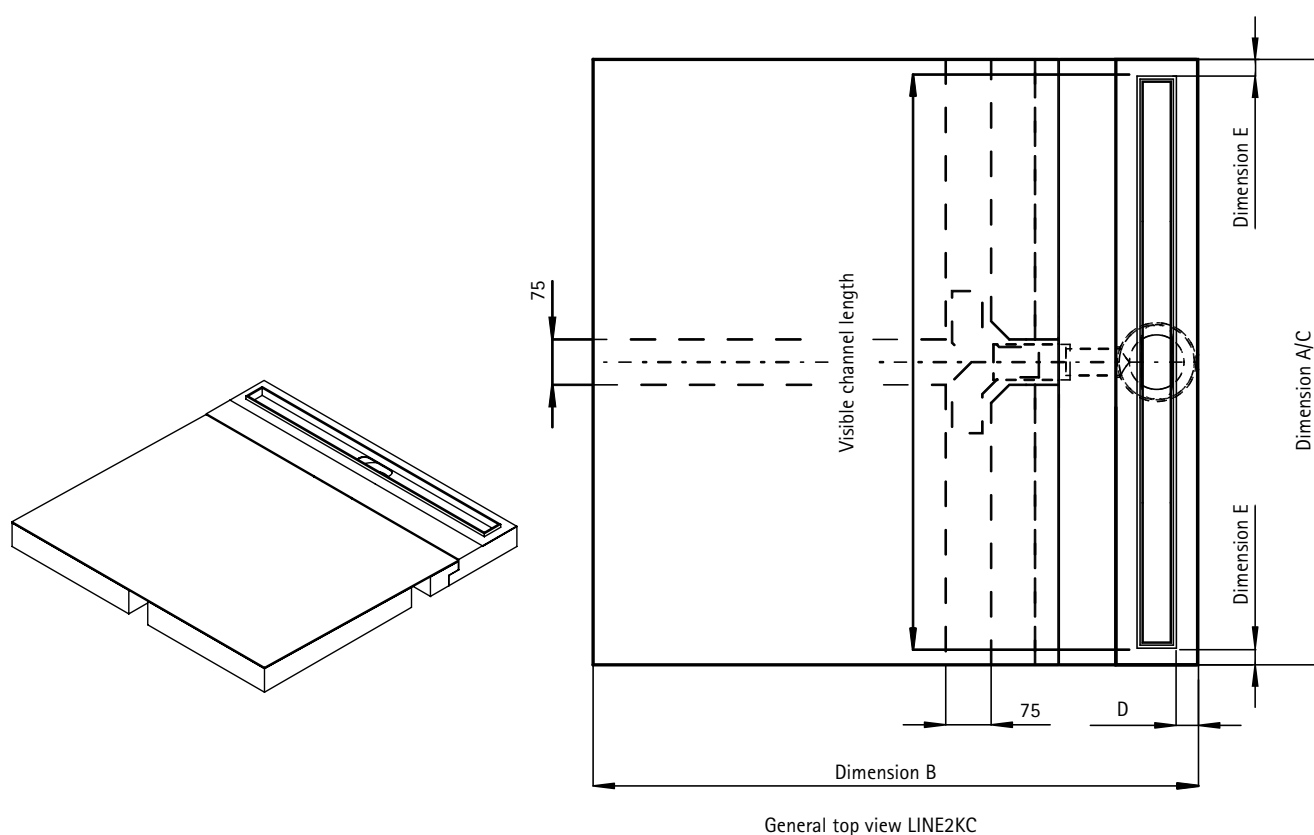
General top view LINE2KC
