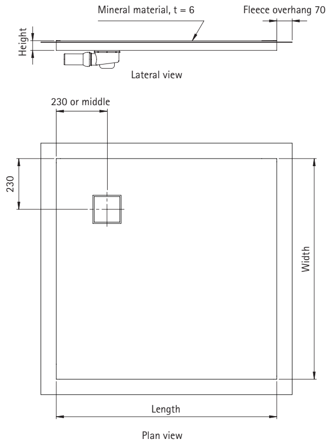
Vertical drain DN 50 Drainage capacity 30.6 l/min
